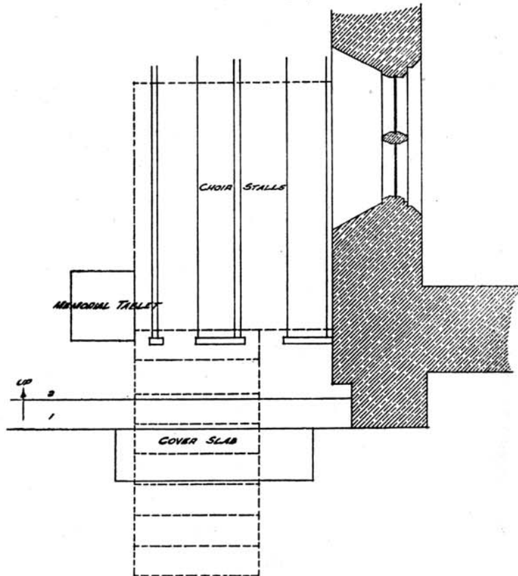
Plan of Part of Chancel, showing position of Vault below.
